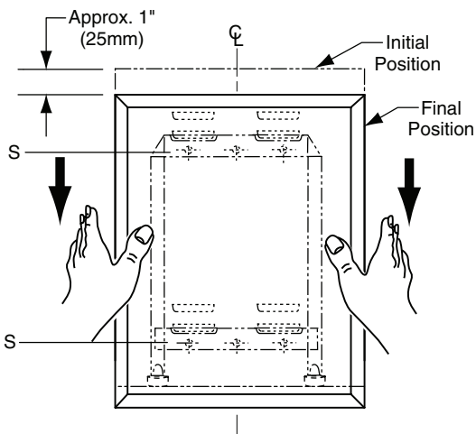
SNAP LOCKING DESIGN (Front View)
